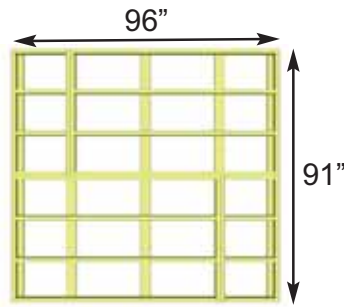
Shed Front Floor Frame
